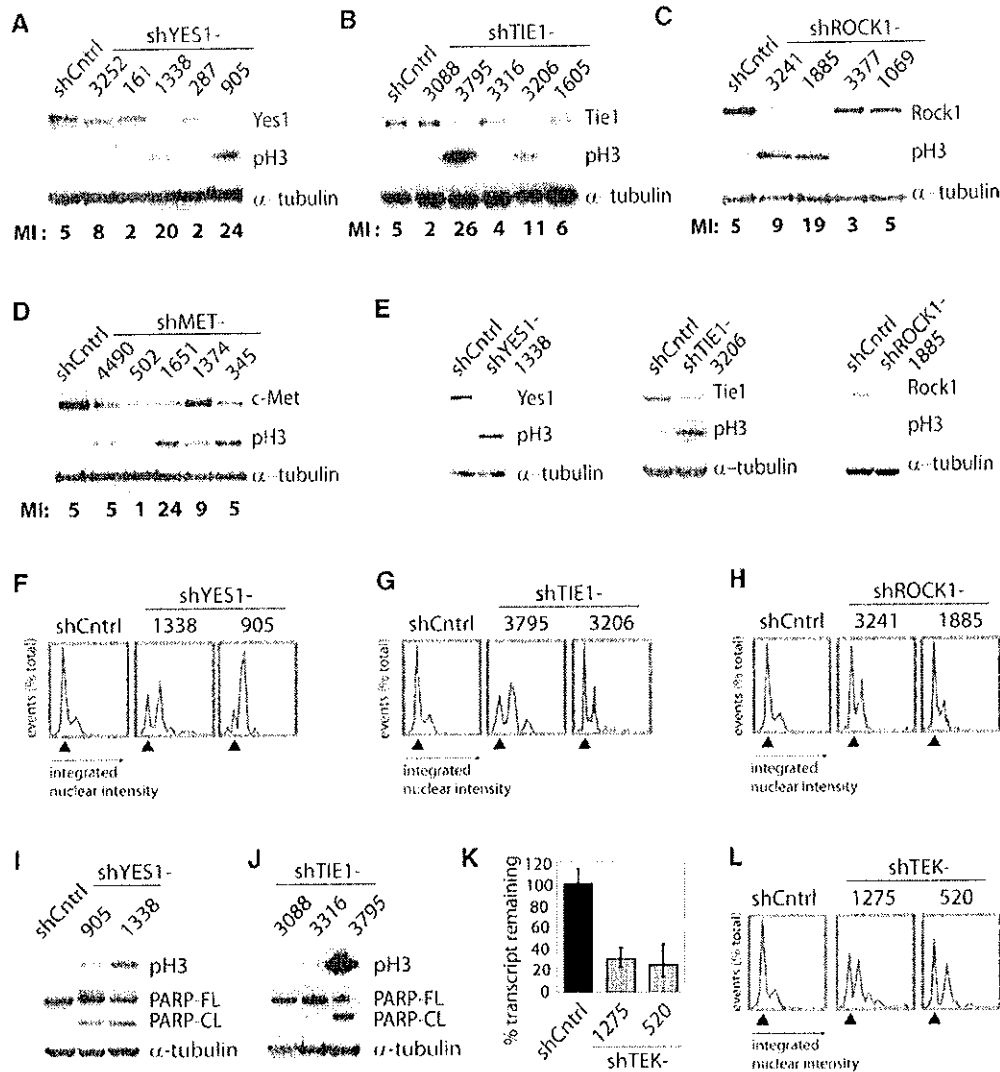
Figure 6. Correlation between Phenotype and Knockdown for Multiple Library shRNAs
