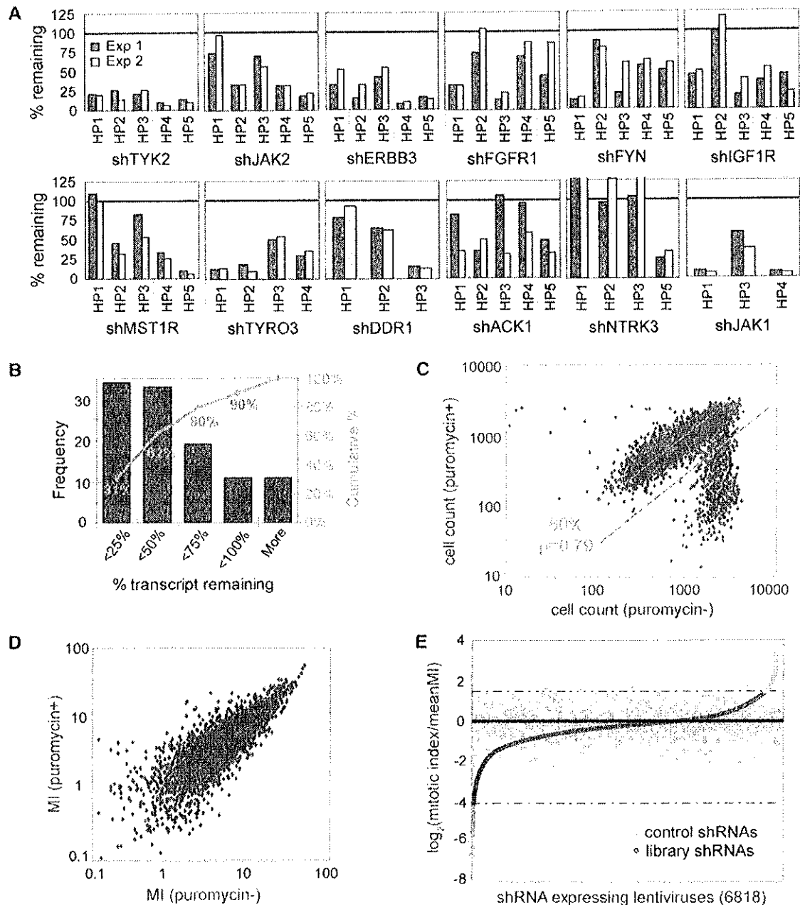
Figure 2. Knockdown Performance of HT-Generated Lentivirus in A549 Cells and Mitotic-Index Screen in HT29 Cells (A) Knockdown performance of lentiviruses representing 54 shRNAs targeting 12 different tyrosine kinases. Transcript levels for duplicate experiments were measured by qRT-PCR and are reported for each shRNA hairpin relative to average transcript levels for two control infections (i.e., an shRNA targeting either lamin A/C or scrambled sequence). Knockdown for the first set of infections is shown by dark blue bars and the second set of infections by light blue bars. (B) Summary of knockdown levels for the duplicate infections of the 54 shRNA viruses from (A). (C and D) Cell counts (C) and MI scores (D) following infection of HT29 cells with TRC1 as determined by automated image analysis with, versus without, puromycin selection. (E) Distribution of MI scores for all shRNA infections. MI scores for library shRNAs are sorted in order of increasing MI and are marked by red (low), blue (normal), and green (high) diamonds. MI scores for 700 control shRNAs are displayed in gray in random order to indicate the background range of MI. High and low MI thresholds for selection of MI hits are marked by the dashed lines.
