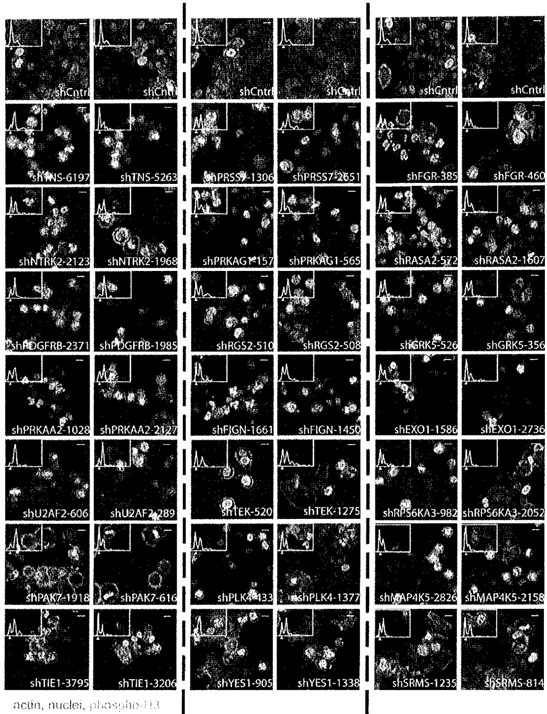
Figure 4. Images of HT29 Cells Infected with shRNAs for 21 Genes that Induce High Mitotic Indices Pairs of images are shown for knockdowns by two distinct shRNA viruses for each hit gene. Scale bars = 10 \mu m. Corresponding DNA content histograms are superimposed as yellow traces in the left corner of each image. The percentage of total events is shown on the vertical axis and the integrated nuclear intensity on the horizontal axis. The control histogram is the average of ten images taken from control infections. The small yellow triangles underneath each histogram indicate the G1 peak in HT29 cells.
