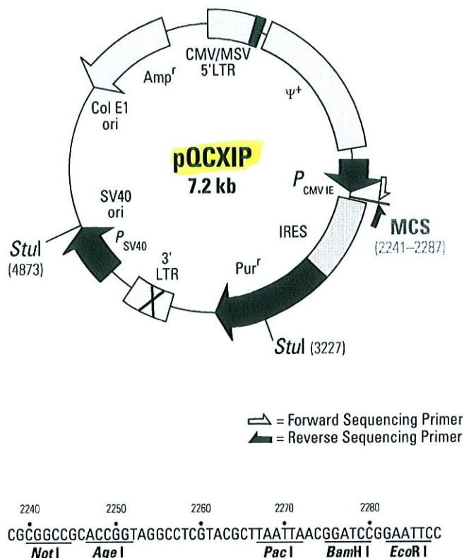
Restriction Map and Multiple Cloning Site (MCS) of pQCXIP Vector. Unique restriction sites are in bold.
