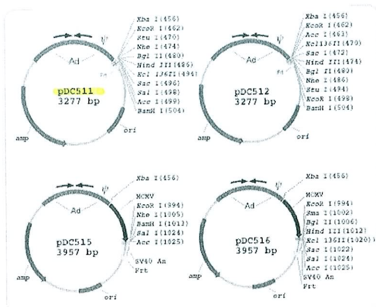
Figure 4 illustrates a set of shuttle plasmids analogous to those shown in Figure 2 but containing frt sites for recombination by the site specific recombinase, FLP, encoded by the yeast 2u plasmid (O'Gorman et al. Science 251, 1351, 1991).
