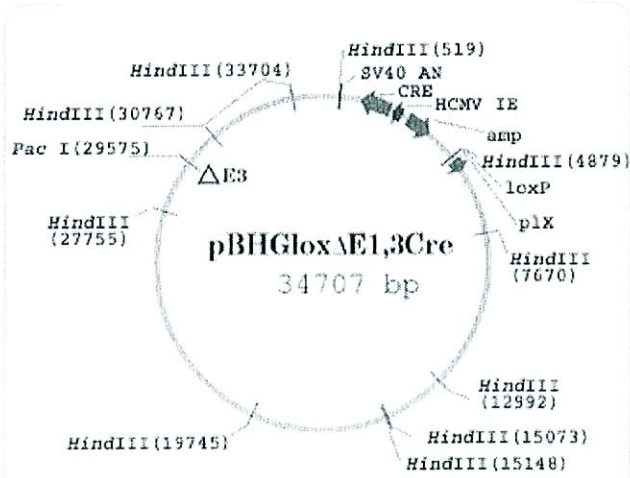
Figure 3. Ad genomic plasmid for construction of Ad vector by Cre-lox recombination
