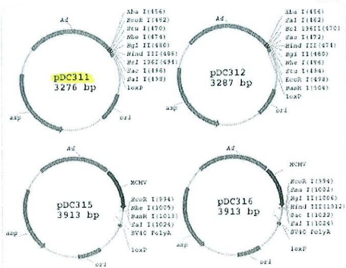
Figure 2. Shuttle plasmids for Cre-lox Ad vector construction
