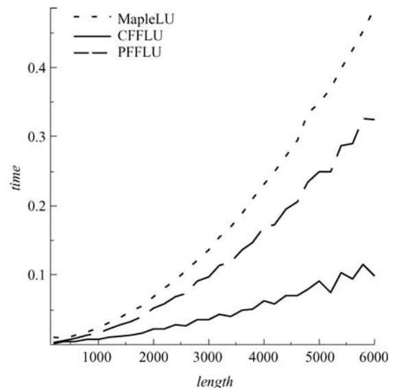
Fig. 3 Time of random integer matrices
