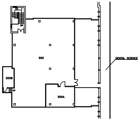
PENTHOUSE FLOOR
